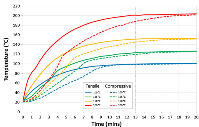
Figure 2. Heat propagation through tensile and compressive PDMS test samples at oven temperatures of 100 °C, 125 °C, 150 °C and 200 °C. Dotted vertical lines indicate selected additional curing times of 13 min (tensile) and 18 min (compression).
