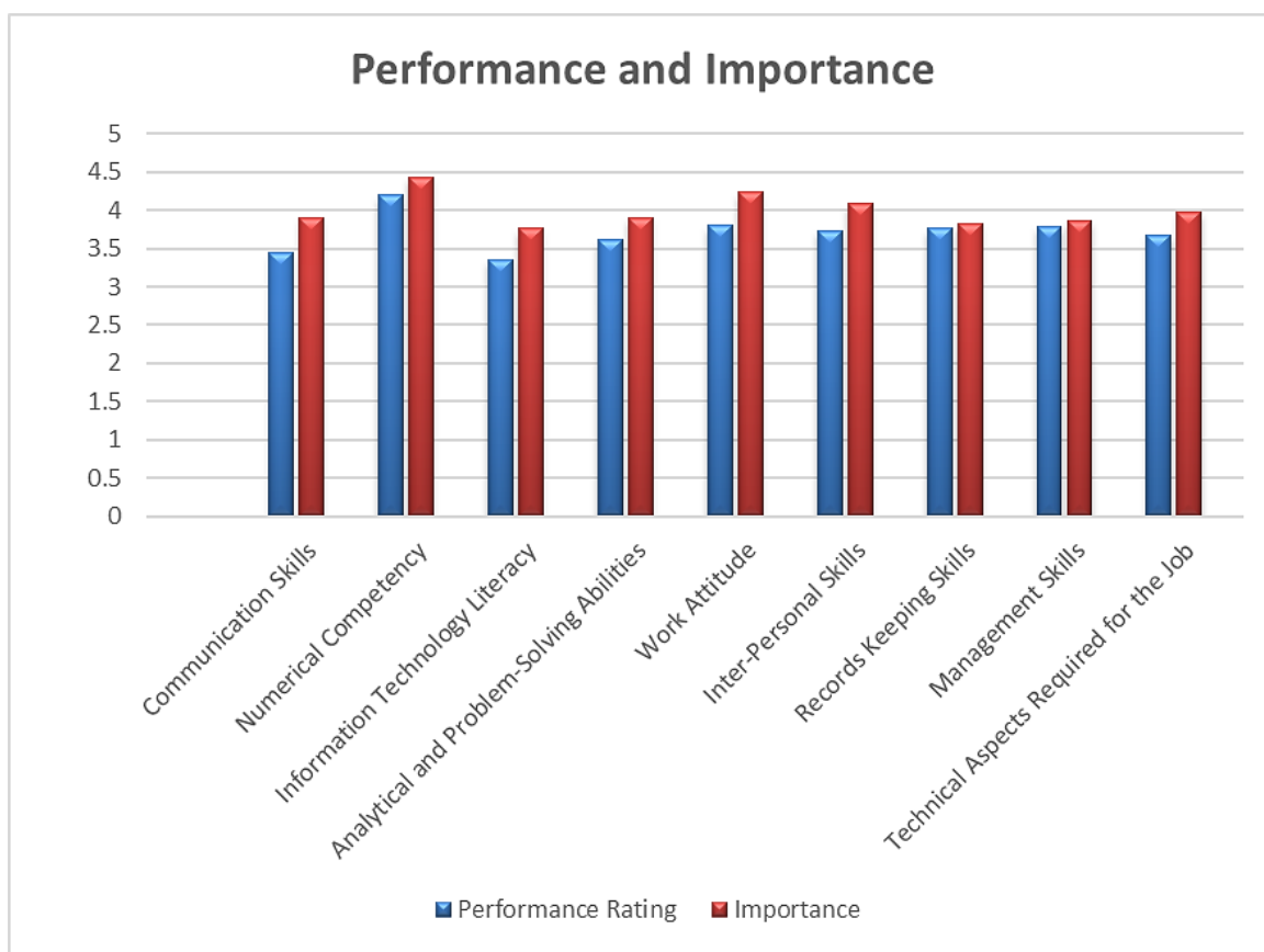
Fig. 1. Performance of BS math graduates and importance rating
