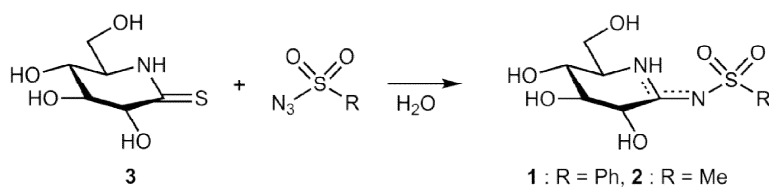
Scheme 2. Protection-free, one-step synthesis of gluconoamidinylsulfones 1 and 2 by the coupling reaction
