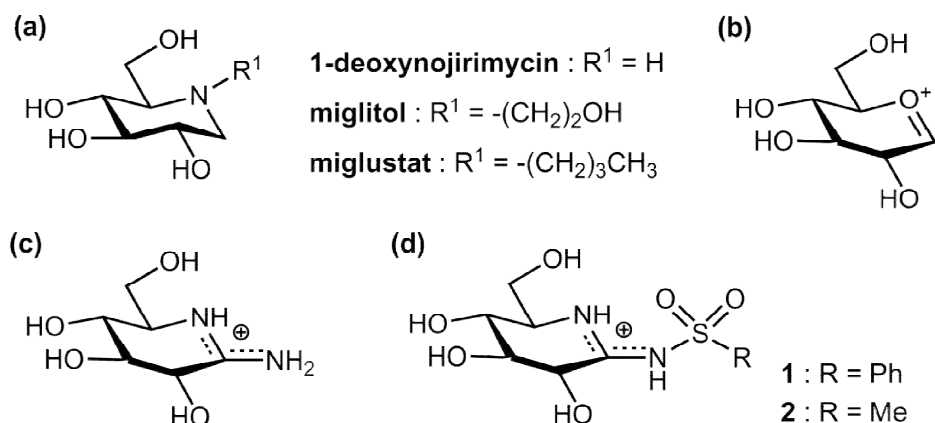
Fig. 1. Chemical structures of (a) 1-deoxynojirimycin, miglitol, and miglustat, (b) a glycosyl oxocarbenium intermediate, (c) a gluconoamidine (protonation form under physiological conditions), and (d) a gluconoamidinylsulfone (protonation form under physiological conditions)
