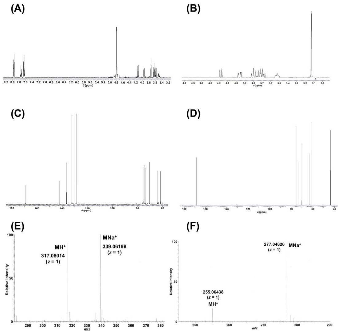
Fig. 2. ^1\text{H} NMR (A and B: 400 MHz in \text{D}_2\text{O} with TSP), ^{13}\text{C} NMR (C and D: 100 MHz in \text{D}_2\text{O} with TSP), and ESI-HRMS (E and F: under the data collection time of 1 min after mass calibration with polyethylene glycol) spectra of gluconoamidinylsulfones 1 (left side) and 2
