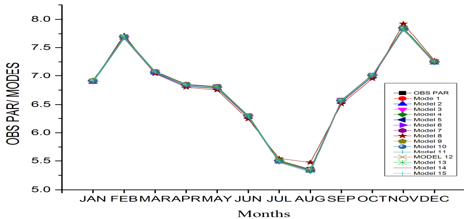
Fig. 1. Comparison between the observed (OBS) and predicted (MODELS) of PAR in MJm -2 day -1 against month for Calabar in all conditions
