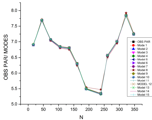
Fig. 2. Comparison between the observed (OBS) and predicted (MODELS) of PAR in MJm -2 day -1 against characteristic day number for Calabar in all conditions
