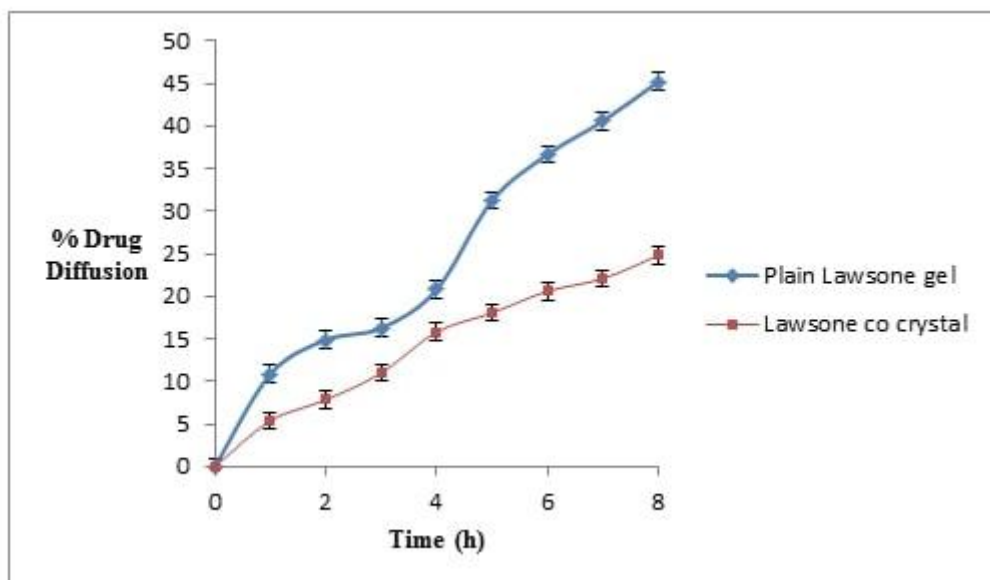
Fig. 8. Drug diffusion of Lawsone loaded co-crystal gel and plain lawsone gel.
