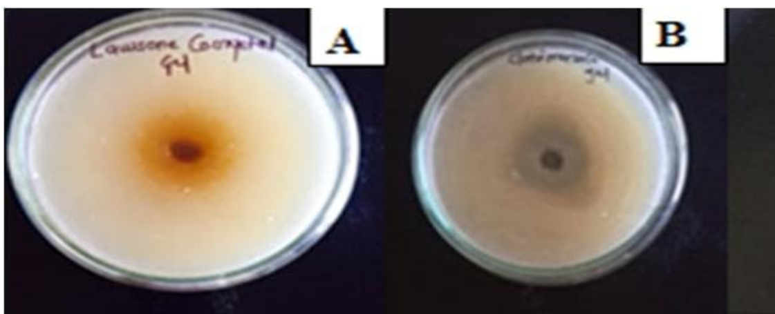
Fig. 9. Zone of inhibition of A-, Lawsone co-crystals loaded gel formulation. B- Marketed Clotrimazole gel (n=3) \pm SD
