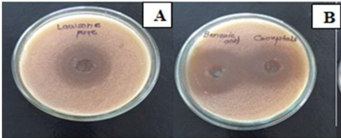
Fig. 6. Zone of inhibition of (A) Pure lawsone, (B) Pure Benzoic acid and Lawsone co-crystal
