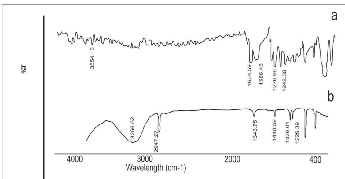
Fig. 1. Fourier transform infrared spectroscopy of a. pure lawsone, b. Lawsone loaded co-crystals formulation
