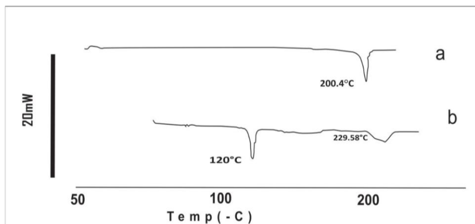
Fig. 2. Differential scanning calorimetry; a. pure lawsone; b: lawsone co-crystals
